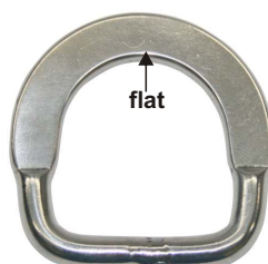
NO.2639 D RING Stainless steel Inside width:30mm(1-3/16") Dia:5mm rod Length:45mm(1-3/4") 200/Box
