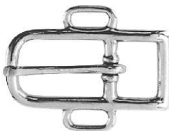
BUCKLE FOR MARATHON Stainless steel NO.2539-32 Inside width:32mm(1-1/4") Length:90mm(3-1/2") NO.2539-36 Inside width:36mm(1-27/64") Length:90mm(3-1/2") NO.2539-40 Inside width:40mm(1-9/16") Length:90mm(3-1/2") 200/Box
