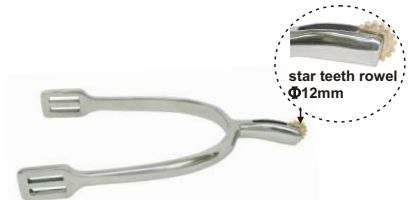
PRINCE WALES SPUR WITH STAR TEETH ROWEL lost wax stainless steel, with teeth star rowel NO.3365-L20S Lady size neck Length:20mm NO.3365-L30S Lady size neck Length:30mm NO.3365-M20S Man size neck Length:20mm NO.3365-M30S Man size neck Length:30mm 50prs/Box
