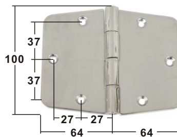
HINGE stamped AISI 316 buff polished ITEM NO. Thickness Weight/g 006132 3mm 340
