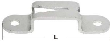
V CLEAT AISI 304 For school masts and booms ITEM NO. L mm 008703 50
