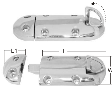
LOCKING DEVICE WITH SPRING
