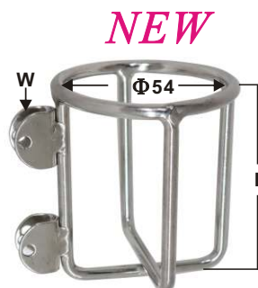
BOAT HOOK HOLDER AISI 304
