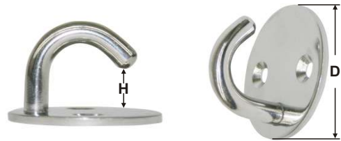
ROUND PLATE HOOKS stamped AISI 304
