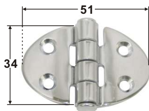
HINGE Stamped AISI 316 Buff polished ITEM NO. Thickness Weight 006134 2mm 30g
